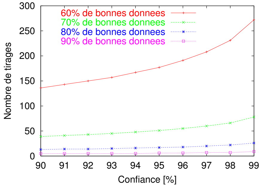
Figure 11: Number of samples that should be processed in order to reach a probability \alpha ('confidence') of encountering at least one sample of 8 good correspondences.
