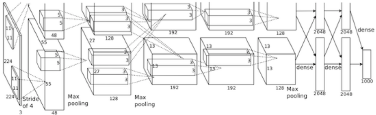
AlexNet Architecture (2010)
