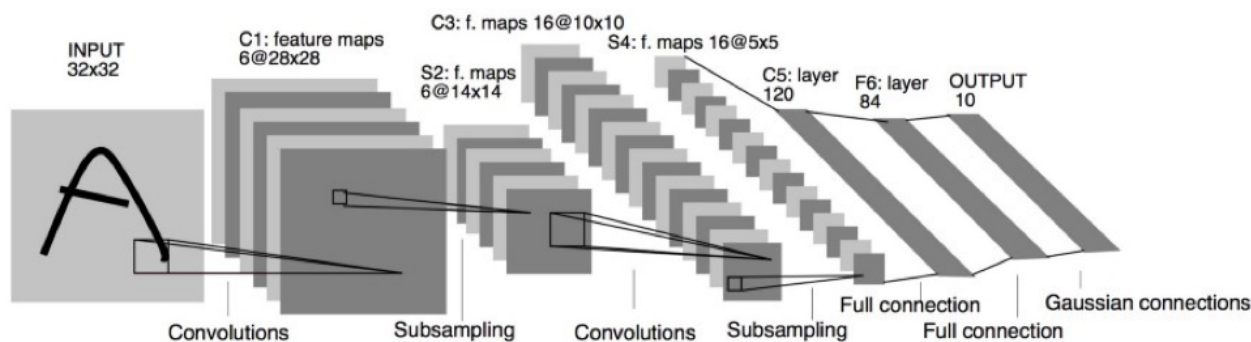
The LeNet5 architecture (1994)
