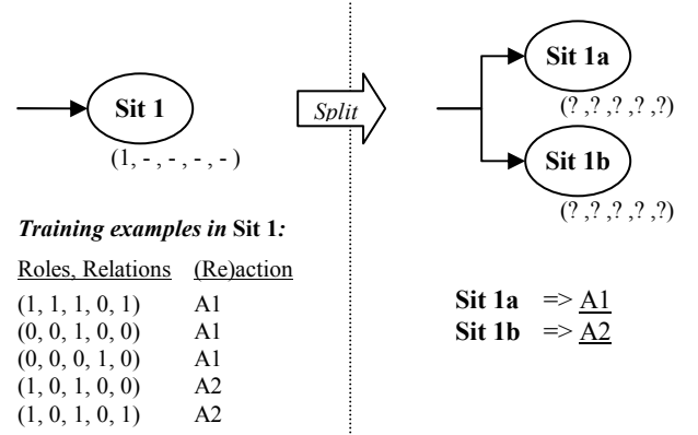
Fig. 3. Splitting Situations. The characteristic roles, relations configuration of Sit 1a and Sit 1b need to be determined (“?”).
