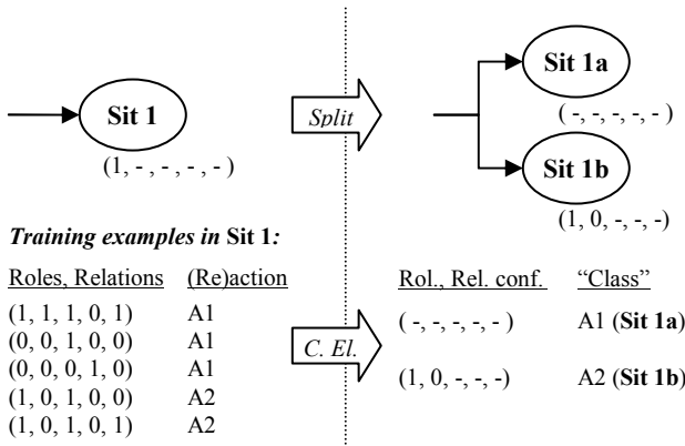
Fig. 5. Splitting Situations with Candidate Elimination algorithm.
