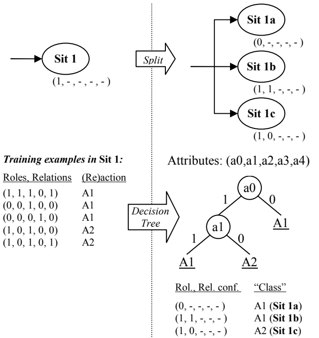
Fig. 6. Splitting Situations with Decision Tree algorithm.
