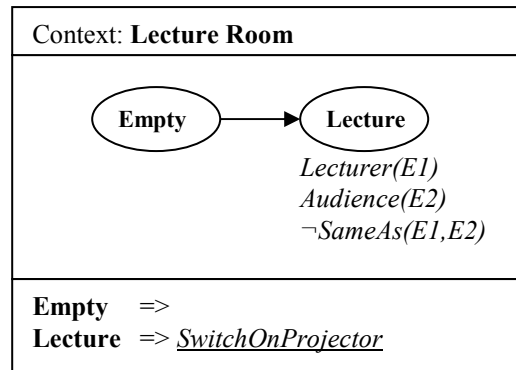
Fig. 1. Example of a context model for a lecture room. Empty and Lecture are the available situations. Lecturer , Audience are the available roles and SameAs the available relation. SwitchOnProjector is a system (re)action. E1 and E2 are entities.
