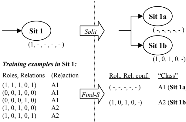
Fig. 4. Splitting Situations with Find-S algorithm.
